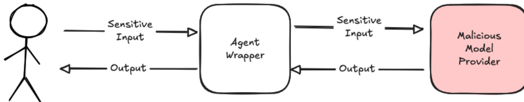
Figure 8: A malicious model provider can steal sensitive user data.
